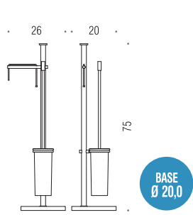
W4935 Piantana con porta rotolo e porta scopino Standing column equipped with paper holder and brush holder
