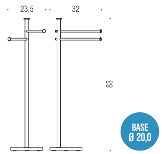
W4936 Piantana con due porta salvietta Standing column equipped with two towel holders
