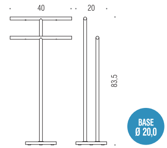
W4938 Piantana con due porta salvietta Standing column equipped with two towel holders
